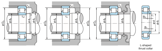
L-shaped thrust collar
