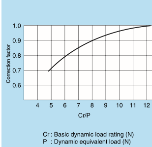
Fig. 8.38.1 Correction Factor for Bearing Load
