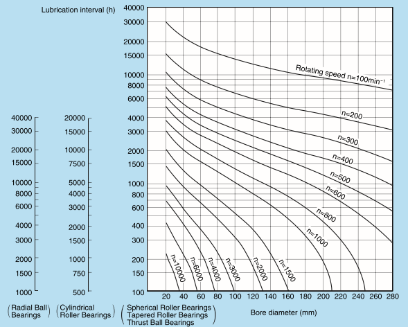
Fig 8.37 Grease lubrication interval
