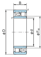
NNU Cylindrical bore
