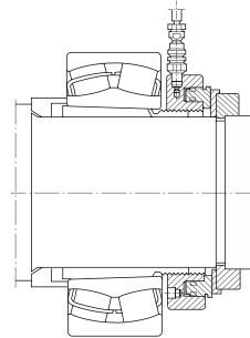
Fig.5. Sleeve thread and special supporting ring
