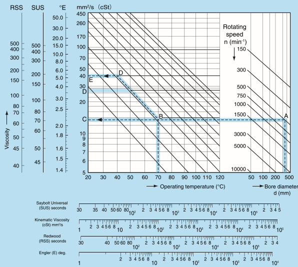
Fig. 8.36 Viscosity-Temperature Line Diagram
