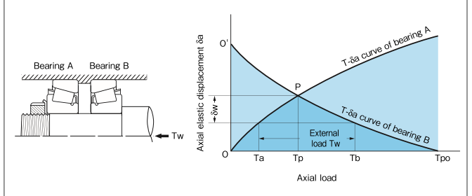
Fig. 8.5 Description of Fixed Position Preloading
