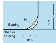
Fig. 8.7 Chamfer Dimension, fillet radius and Shoulder Height
