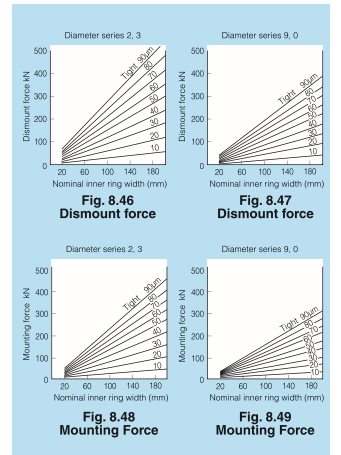
Fig. 8.46 Dismount force , Fig. 8.47 Dismount force , Fig. 8.48 Mounting Force , Fig. 8.49 Mounting Force
