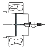
Dismounting Bearing with Oil Injector Fig. 8.56
