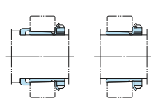
Fig. 8.14 Adapter Sleeve Mounting
