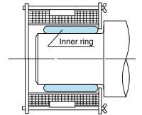
Fig. 8.55 Inner Ring Removal with Induction Heater
