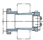
Fig. 8.17 Withdrawal Sleeve Mounting
