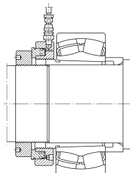
Fig.3. Sleeve thread
