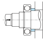
Fig. 8.50 Dismounting Bearing Using Press
