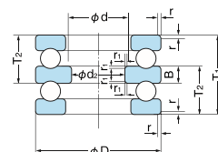
Fig 4.4 Double-direction Thrust Ball Bearings
