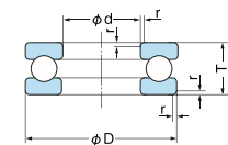
Fig 4.3 Single-direction Thrust Ball Bearings
