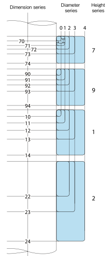
Fig 4.7 Graphical Representation of the Dimension series of Thrust Bearings (except diameter 5 series)
