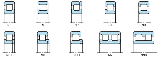
Fig 1. Cylindrical Roller Bearing Configurations
