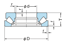
Fig 4.5 Spherical Roller Thrust Bearings
