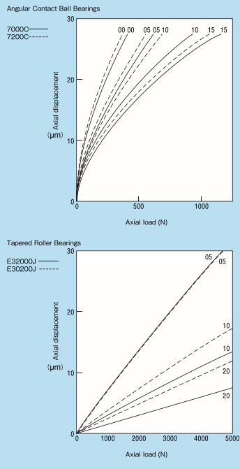
Fig. 8.4 Axial Load and Axial Displacement
