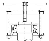
Fig. 8.53 Dismounting Bearing with Special Puller
