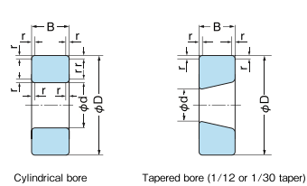
Fig 4.1 Radial Bearings (except Tapered Roller Bearings)
