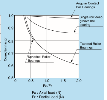
Fig. 8.38.2 Correction Factor for Fa/Fr
