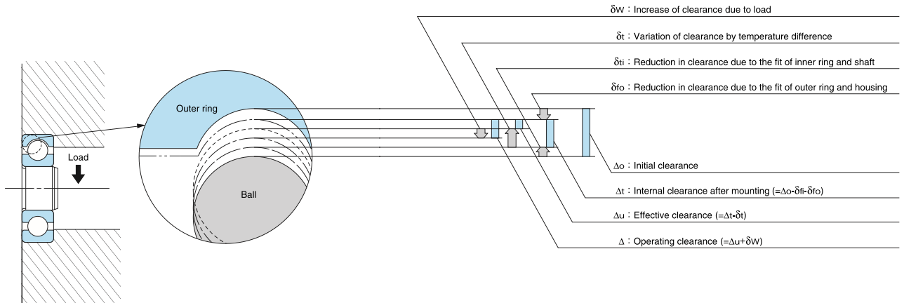
Fig. 8.3 Radial clearance of bearing
