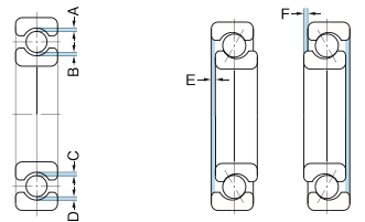
Fig 6.1 Radial internal clearance = A+B+C+D
