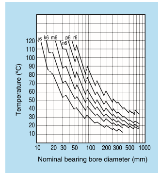
Fig. 8.44 Relationship between Required Bearing Temperature and Fit
